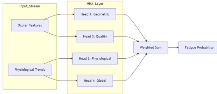
Figure 3 Parallel Reasoning in Multi-Head Attention (MHA)
