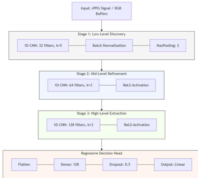
Figure 5 1D-CNN Architecture. This three-stage pipeline distillates high-dimensional physiological features from temporal RGB buffers.
